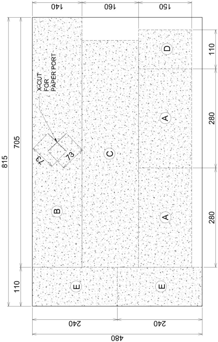
Damping Material Cut Pattern (dimensions in mm)
